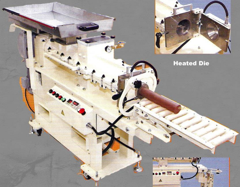
Feed Tray with Safety Screen
