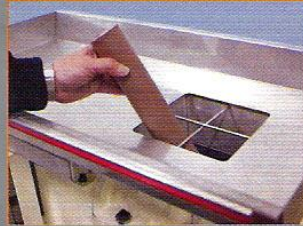
Feed Tray with Safety Screen
